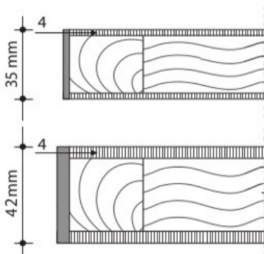
PROFILE DETAIL
